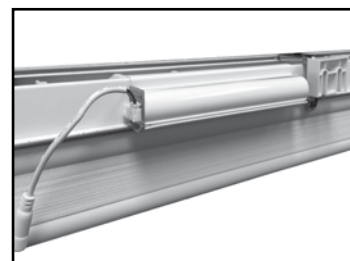
Snap-On external battery for TDBU shades under 36" in width. Spacer block also required for outside mount.
